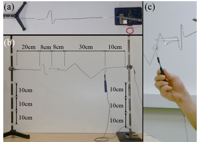
Figure 2 – Experiment set-up. (a) The buzz-wire top view, (b) the buzz-wire frontal view, (c) a participant passing the loop on the buzz-wire.
