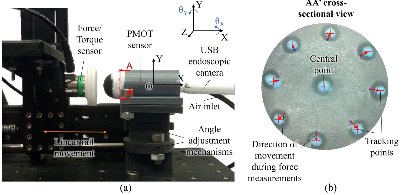
Fig. 3. (a) Experimental setup: A Force/Torque sensor mounted on a robotized linear rail exerts forces on the elastic membrane of our sensor prototype. As a result, (b) the projected locations of the tracking points are visually monitored and analyzed.
